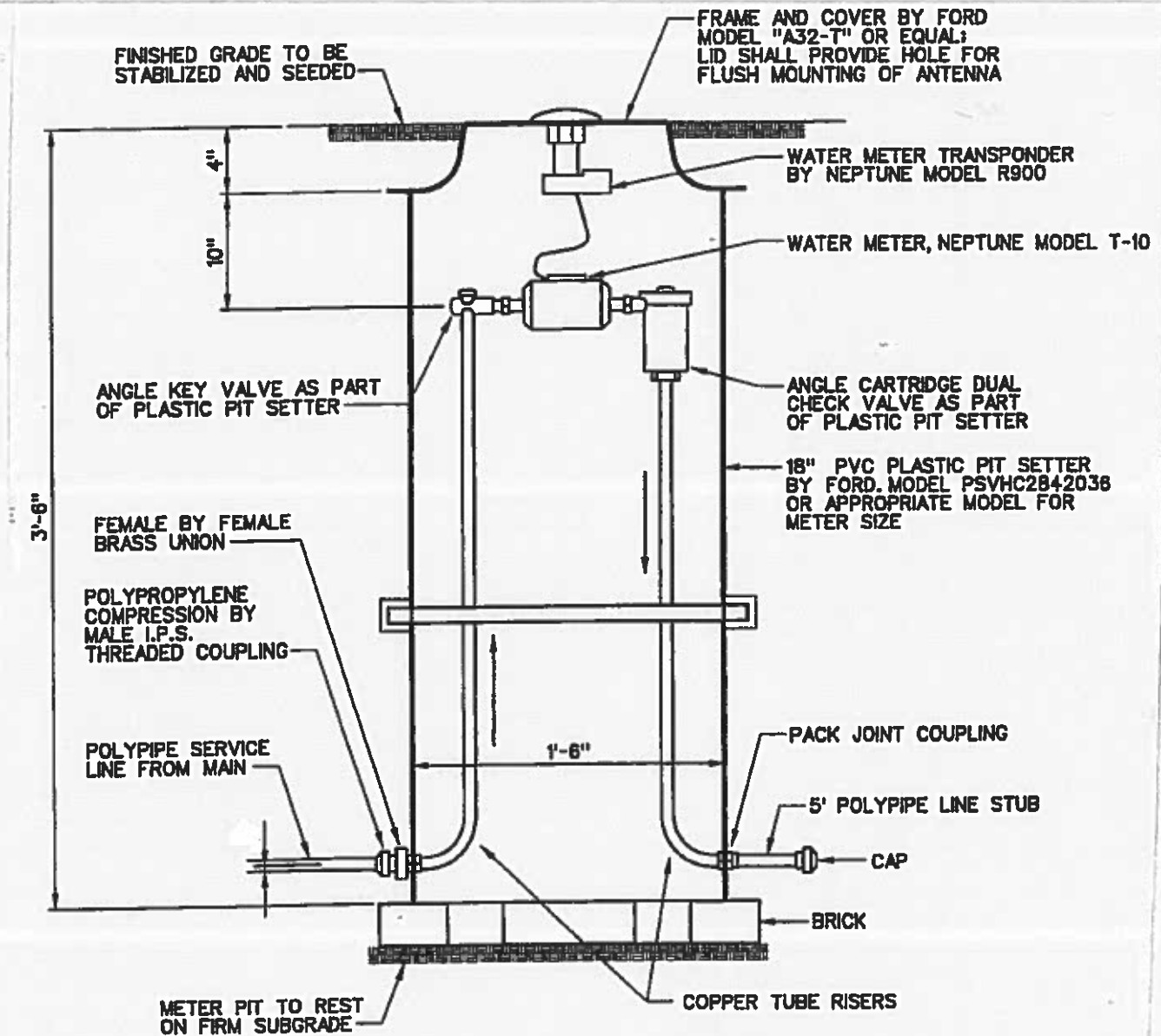
METER PIT DETAIL
